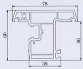
Outward Sash-SF78C
