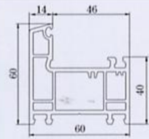
Frame-BR60
